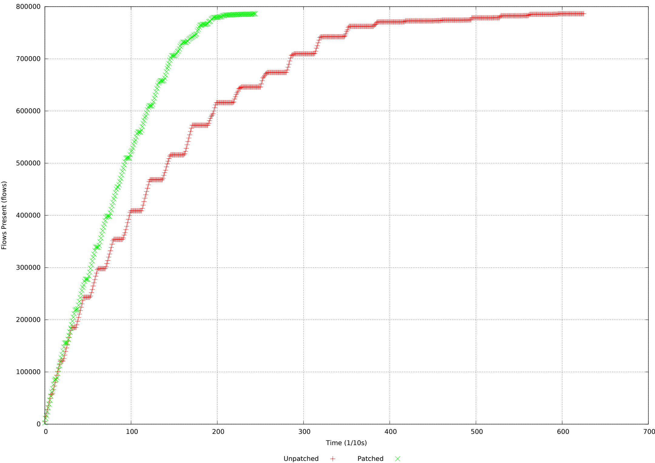
Flows Present vs Time - 768Kflows - 450,000 128 Byte Packets/s
